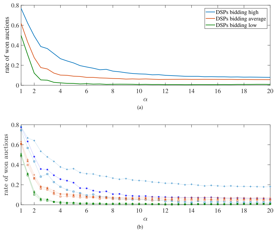
Fig. 16. Evolution of the rate of won auctions for different values of \alpha (from 1 to 20 in steps of 0.5) and \lambda = 0.05 . We consider 20 DSPs with different behaviors (bidding high, average and low). For each value of \alpha , we repeat the experiment 20 times. The results are depicted averaged in (a) for each type of DSP. In (b), we illustrate results of percentiles 3 (using '+'), 50 (using '*') and 97 (using '□'). For these experiments, bid requests for the different types of DSPs are generated using a Gaussian distribution.
